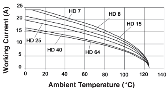
HD CRIMP MACHINE: 1.5 mm 2 (16 AWG)
