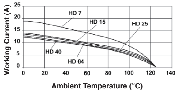
HD STAMPED & FORMED: 1.5 mm 2 (16 AWG)
