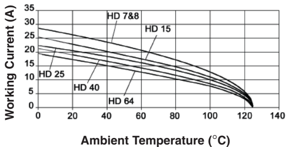
HD CRIMP MACHINE: 2.5 mm 2 (14 AWG)
