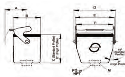
EPIC® HA 3/4 Cable Coupler Hood; Single Lever
