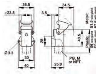
EPIC® HA 3/4 Surface Mount Base; Single Lever
